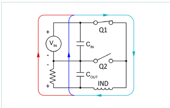
Figure 64 Current flow: Q1 closed
